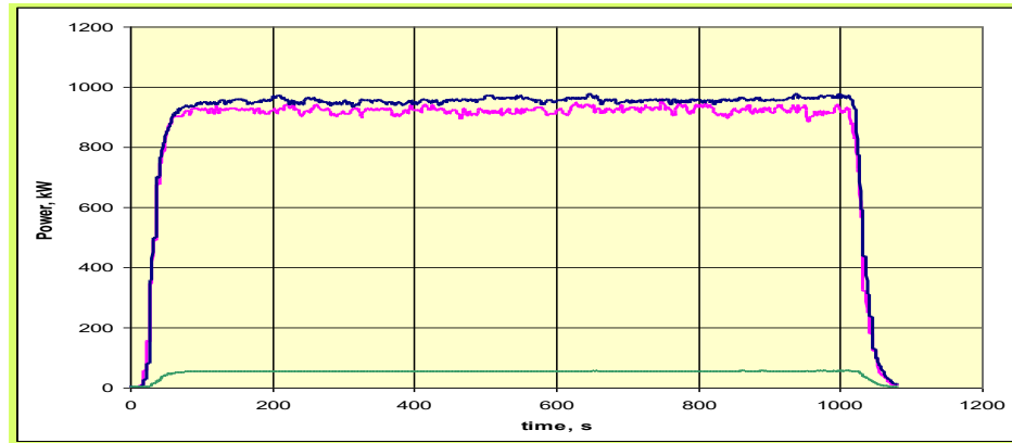
V-11: Power calorimetry in the 1MW/1000s pulse
